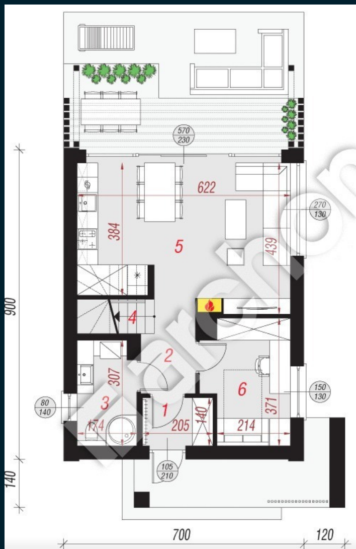
PARTER
